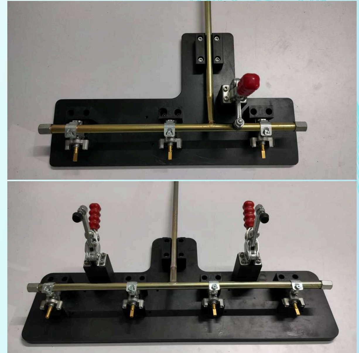
GAS PIPE HOLDING FIXTURE
