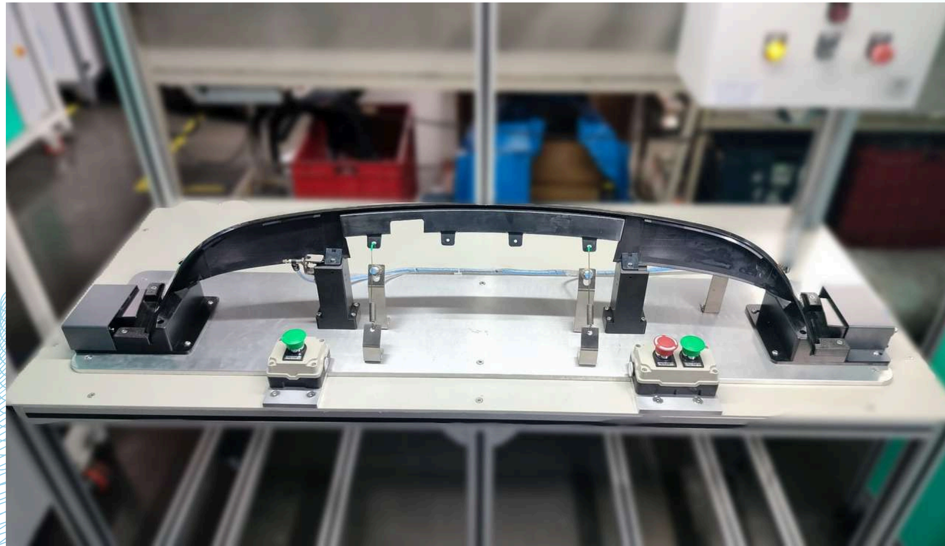
SPOILER COOLING FIXTURE
