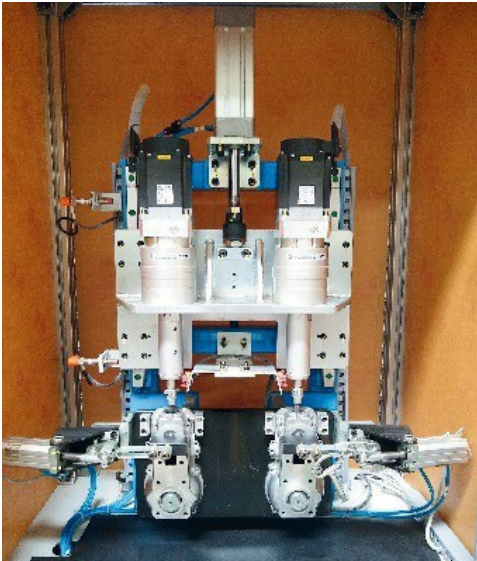
Servo Based Torque Tightening Machine
